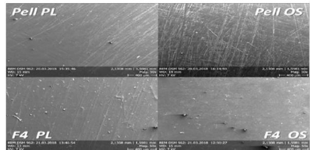
Figure 4: SEM micrographs (50X) of Pellethane 2363-80A and sample F4 after 3 months of storage at 37 °C in PL and in OS.
