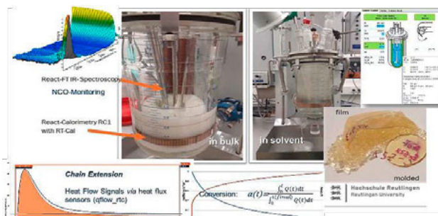
Figure 1: Experimental setup of the real-time monitoring polyurethane formation in TSiPCU production.
