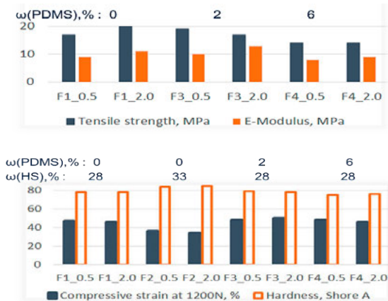
Figure 2: Mechanical properties of the dried F 1 - 4: (a) tensile test ( sd = 0.2-0.6); (b) compression test under application-relevant loading ( sd = 0.1-0.4)
