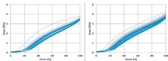
Figure 3: Cyclic tensile testing the sample F1 dried (right) and after 1 month of storage at 37 oC in PL solution (left). For fatigue life estimation of the test-specimens the hysteresis ratios (hr, %) of 4th, 10th and 100th cycles were calculated.
